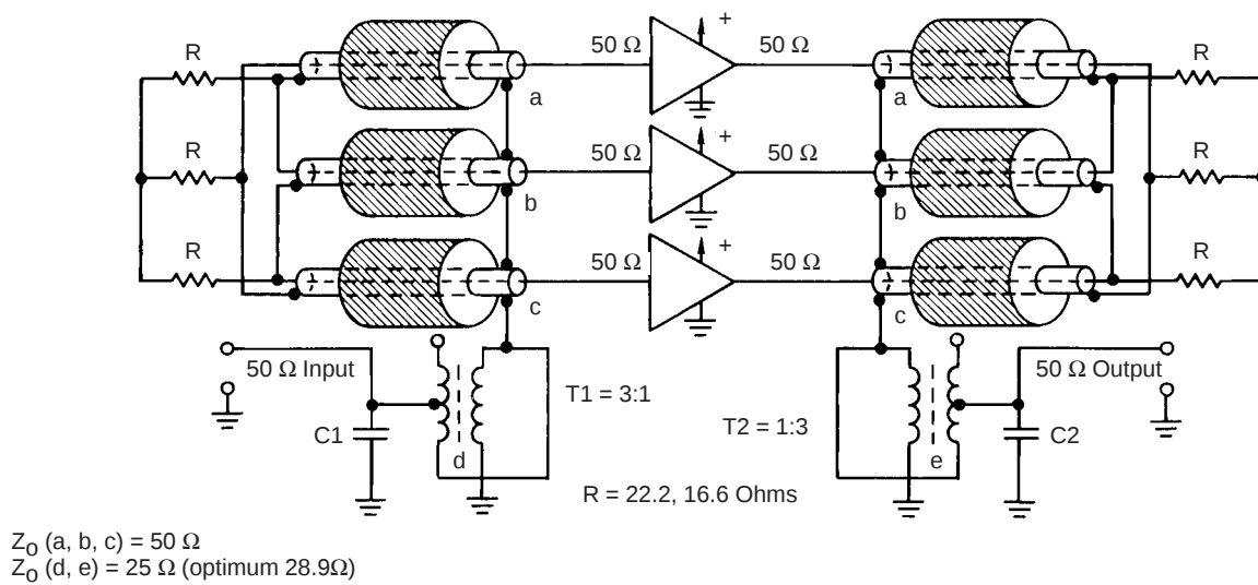
Figure 9. Three-Port Hybrid Arrangement
